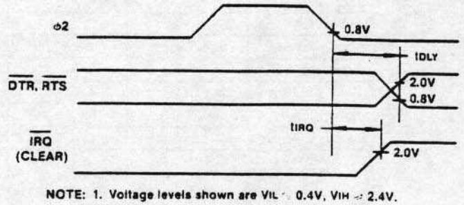
Figure 4. Interrupt and Output Timing
