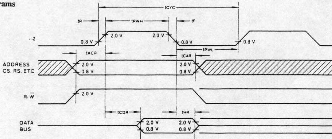
Figure 1. Read Timing
