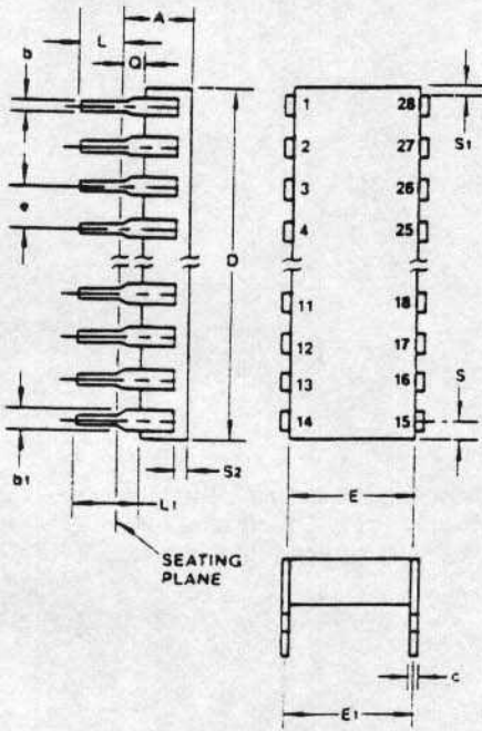
Ceramic Package
