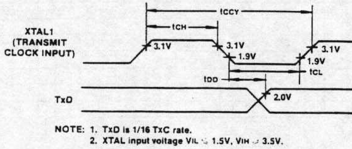
Figure 3. Transmit Timing External Clock
