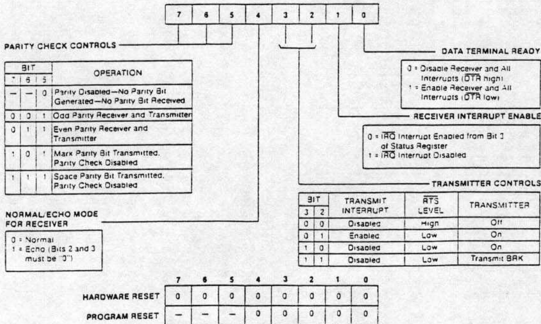
Figure 7 - Command Register Format
