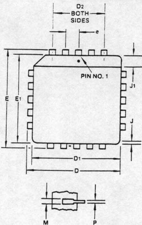
Plastic Leaded Chip Carrier
