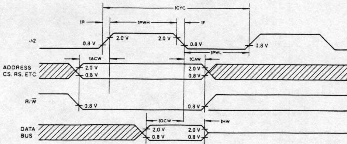
Figure 2. Write Timing
